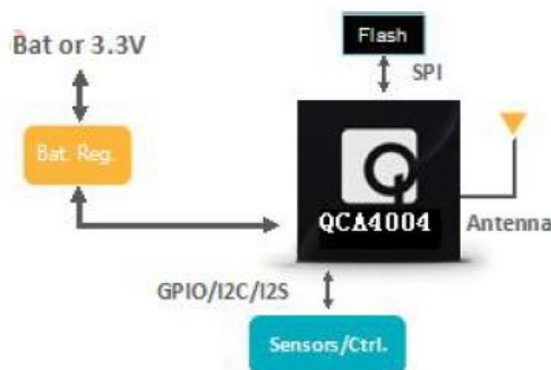
Serial to Wi-Fi SoC Solution
